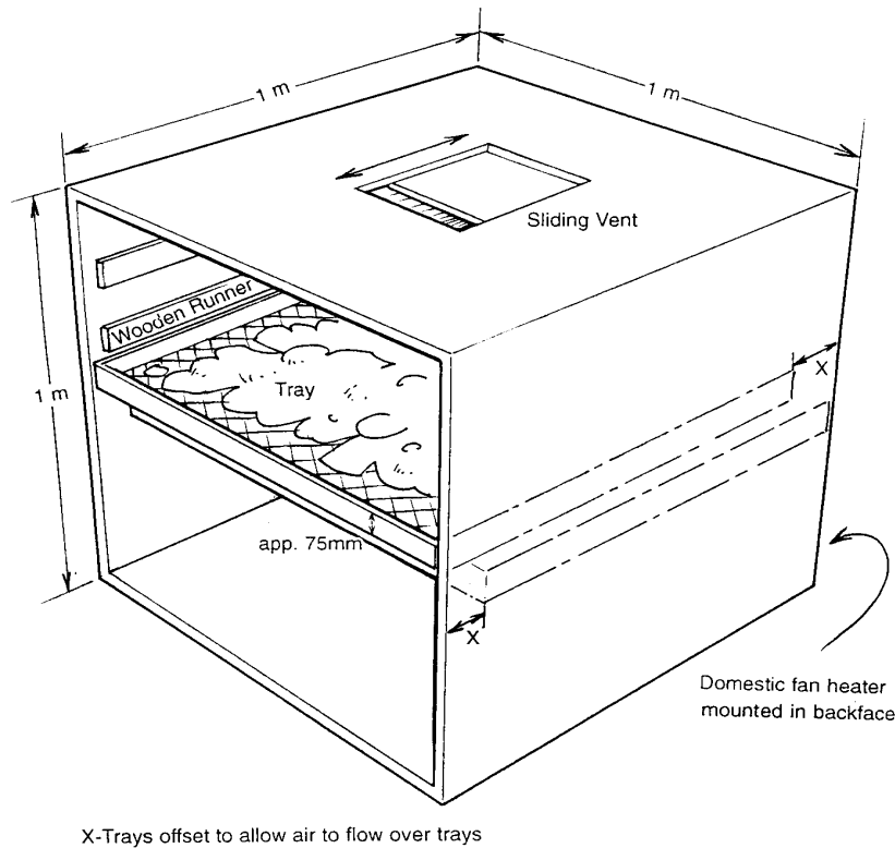
Figure 5: Small electric dryer. The air should follow a zigzag path.
