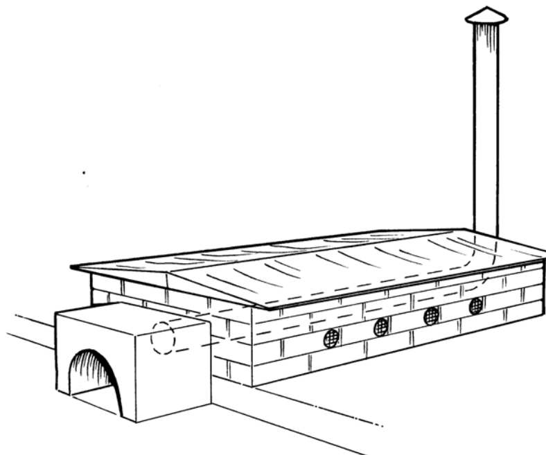
Figure 4: McDowell mixed dryer
