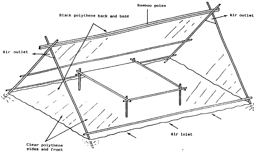
Figure 1: Typical tent solar dryer
